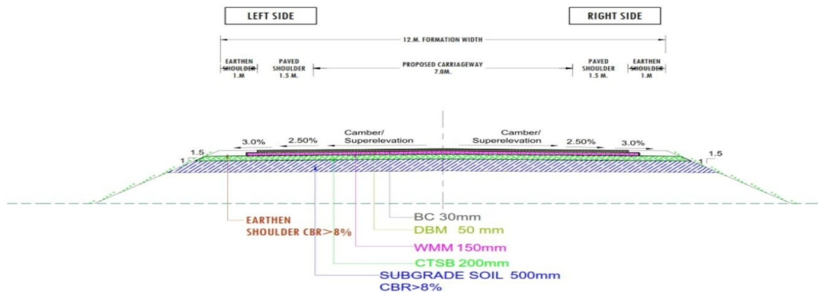
Fig. 2.9 Modified As per IRC SP 73: 2018
