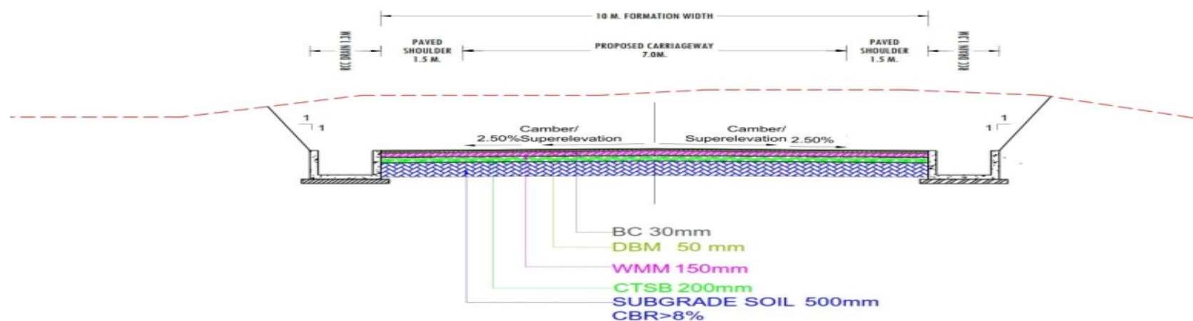
Fig. 2.9 Modified As per IRC SP 73: 2018
