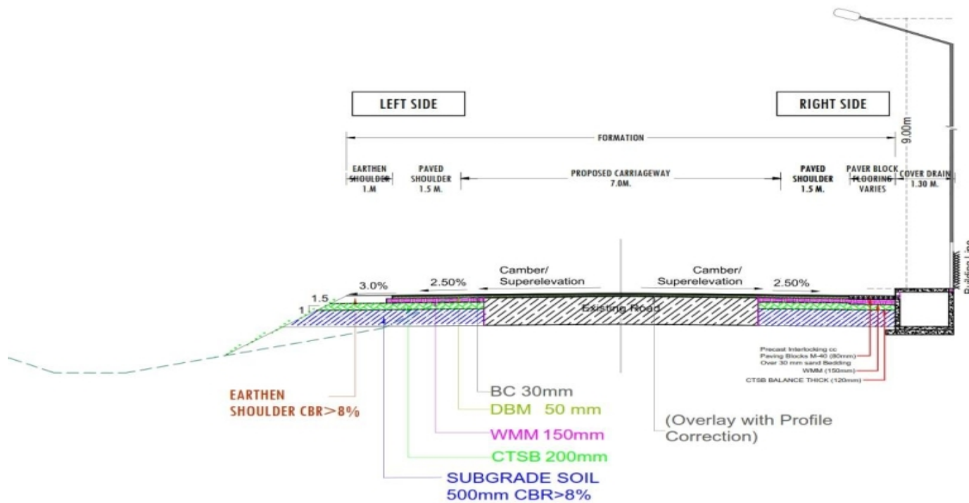
Fig. 2.9 Modified As per IRC SP 73: 2018
