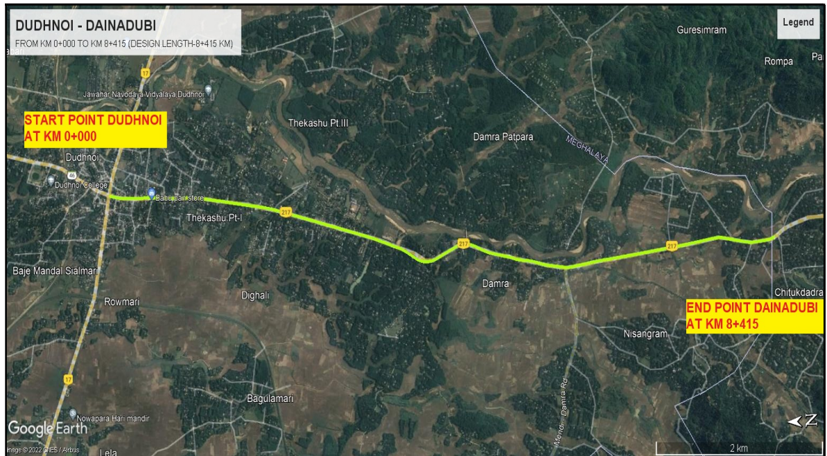
Project Alignment (In green colour) on Satellite Image.
