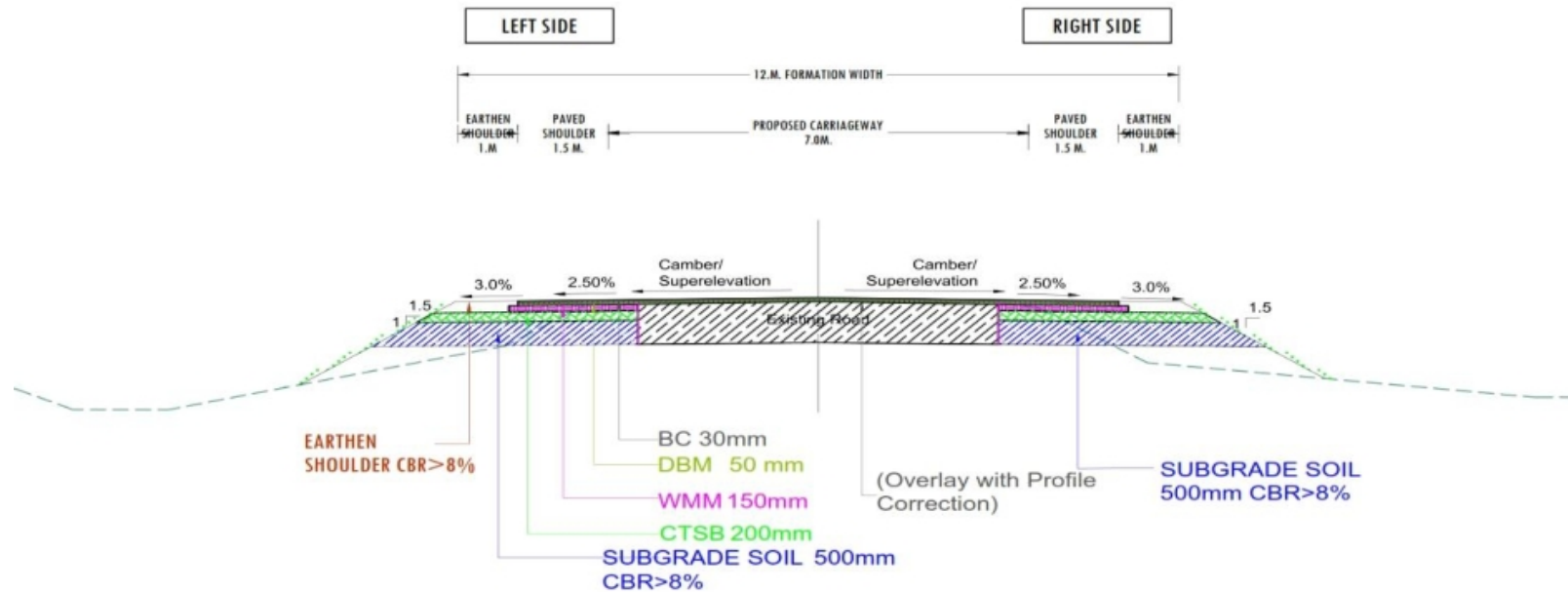
Fig. 2.9 Modified As per IRC SP 73: 2018
