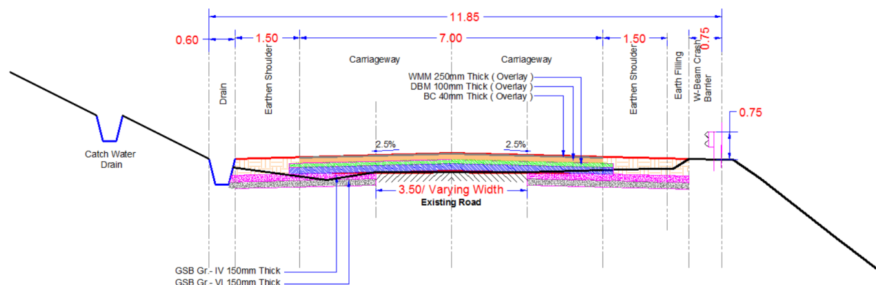
Figure B1: TYPICAL CROSS SECTION 1
