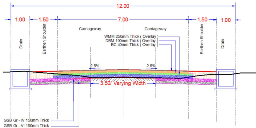
Figure B3: TYPICAL CROSS-SECTION 2A
