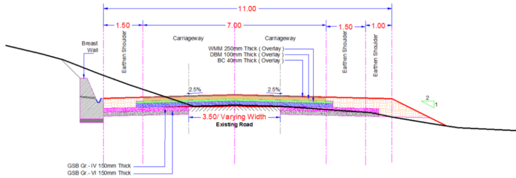
Figure B6: Typical Cross-section 4
