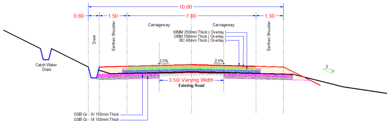
FigureB 4: Typical Cross-section 3
