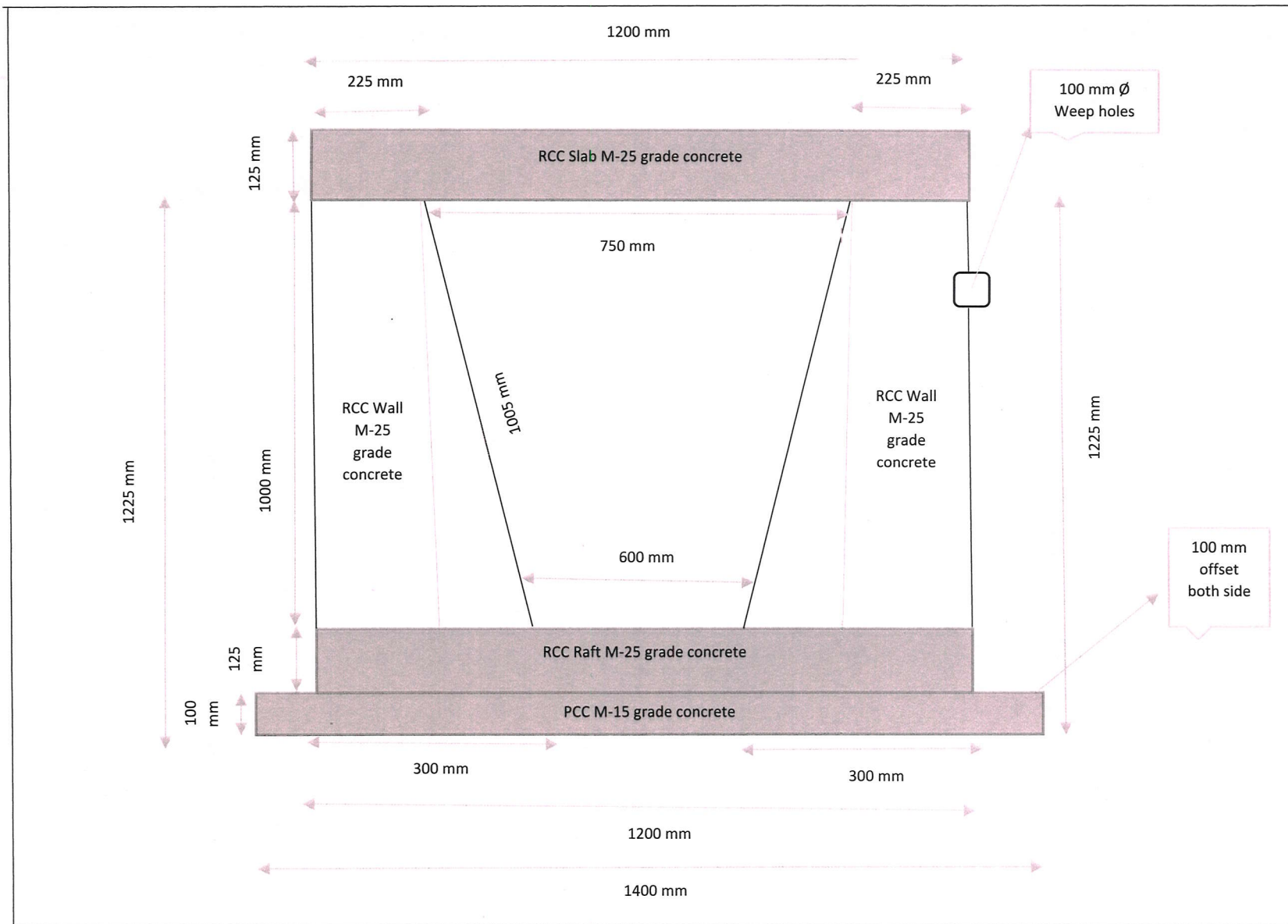
General Arrangement Drawing of runoff water RCC Drain along NH-244 passing through Urban area of Kishtwar city
