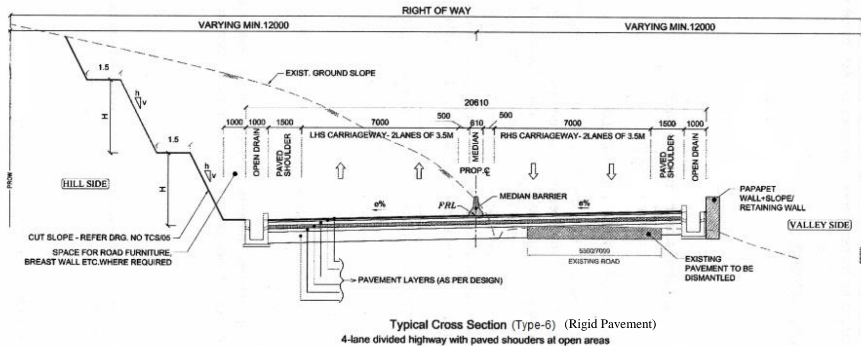
Fig 2.14: Typical Cross-Section
