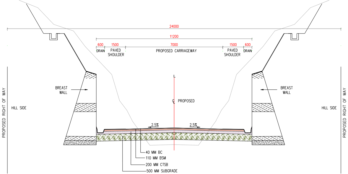
TCS-VII Two Lane With Paved Shoulder Realignment (Both Side Hill Section)
