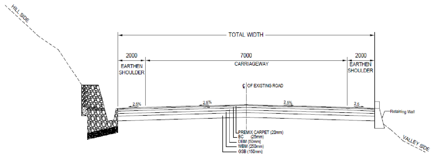
TCS -1 TYPICAL CROSS SECTION FOR EXISTING ROAD (AT THROUGH CUTTING PORTION)
