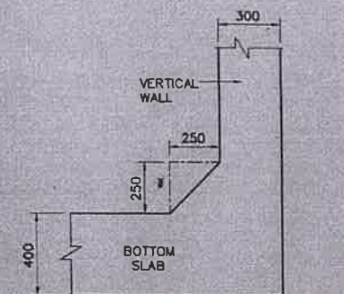
TYPICAL DETAIL OF HAUNCH SCALE 1:30
