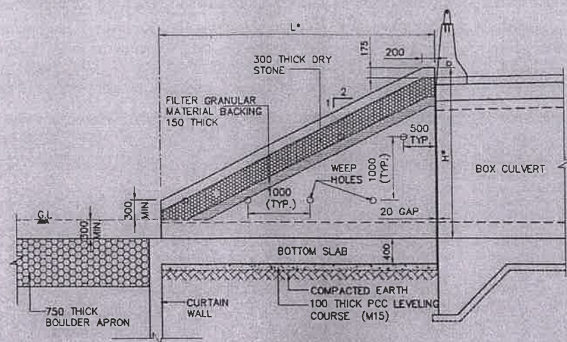
SECTION A-A SCALE 1:75
