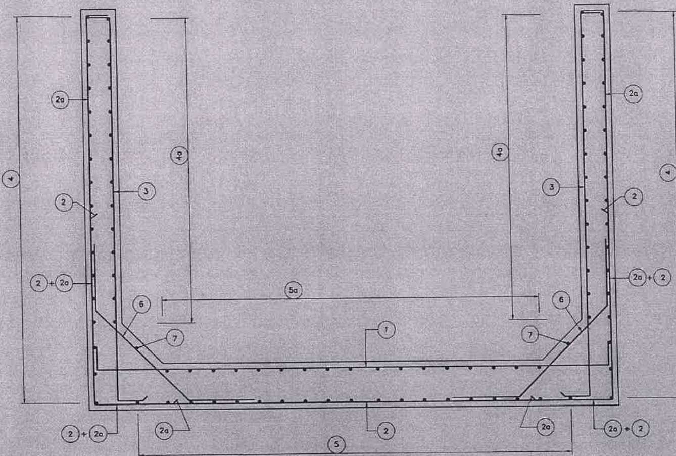
REINFORCEMENT DETAIL OF U-TROUGH SCALE 1:30
