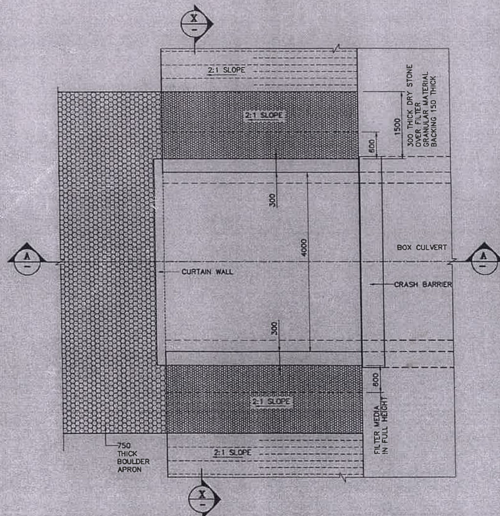
PLAN OF U-TROUGH FOR CULVERTS WITHOUT CUSHION (FOR ORIENTATION REFER CULVERT DRAWING) SCALE 1:75
