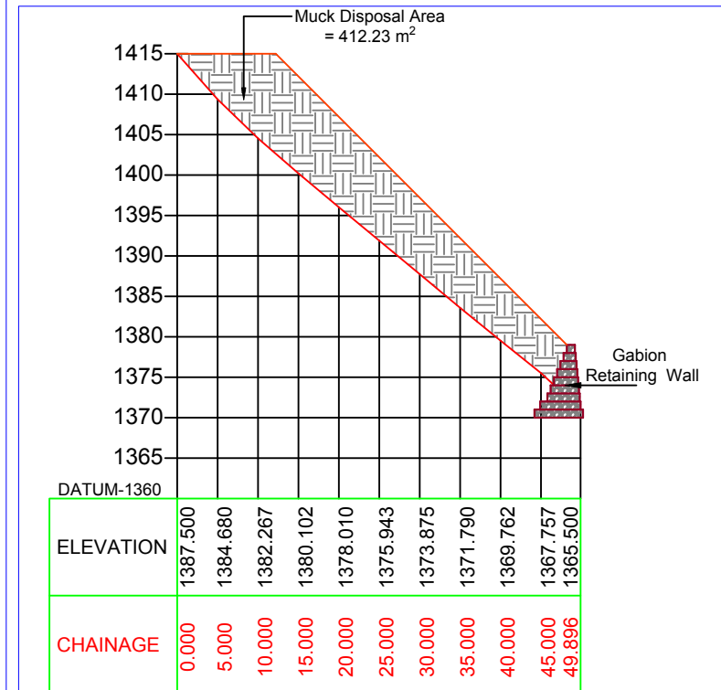
Section At -3 Scale-1:750
