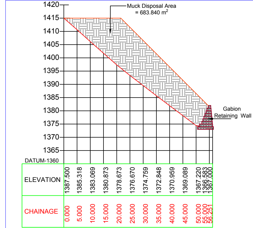
Section At -2 Scale-1:750
