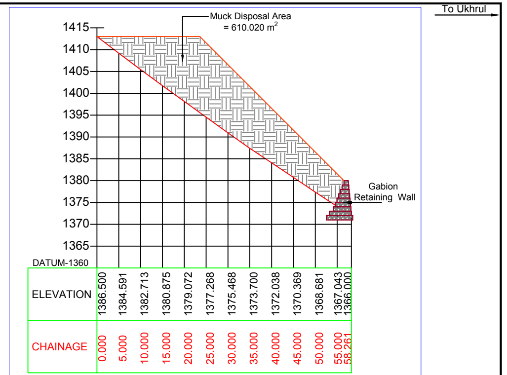
Section At -1 Scale-1:750
