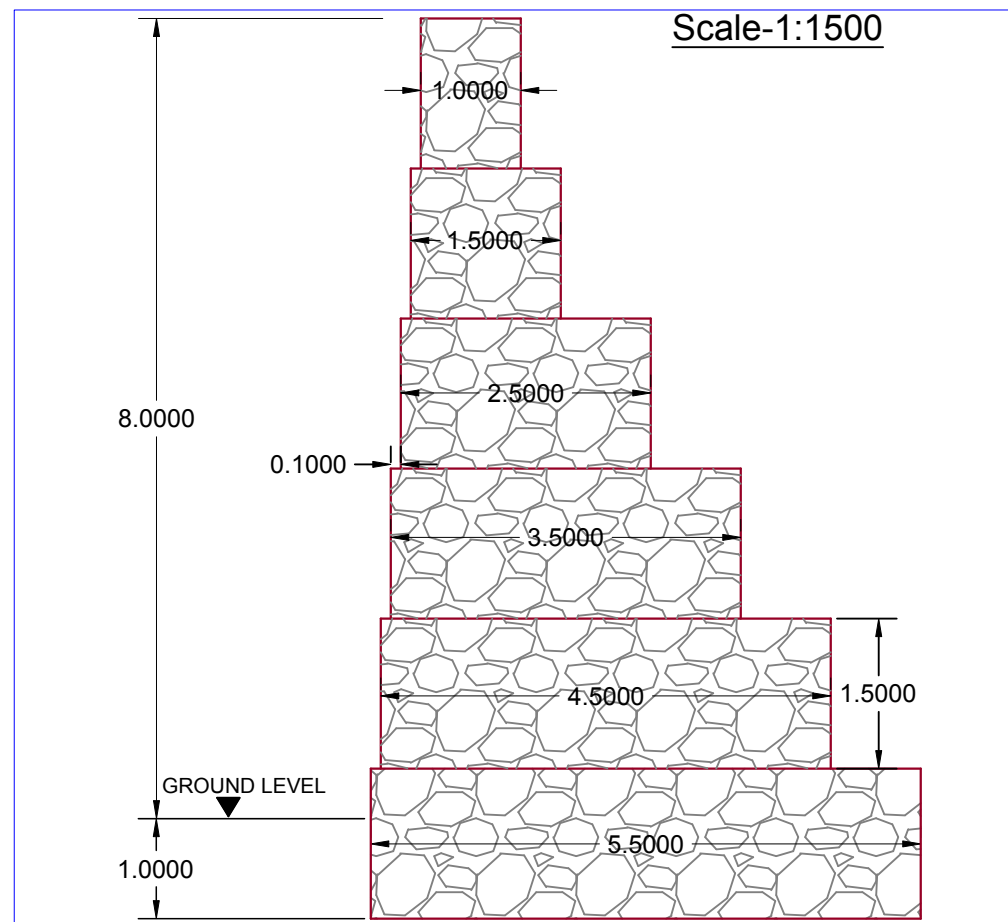
Cross Section of Gabion Retaining Wall (9.0M HT.)
