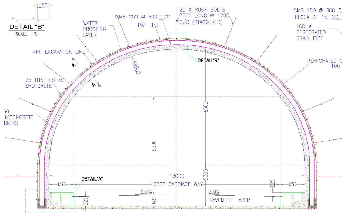
Typical section of Tunnel
