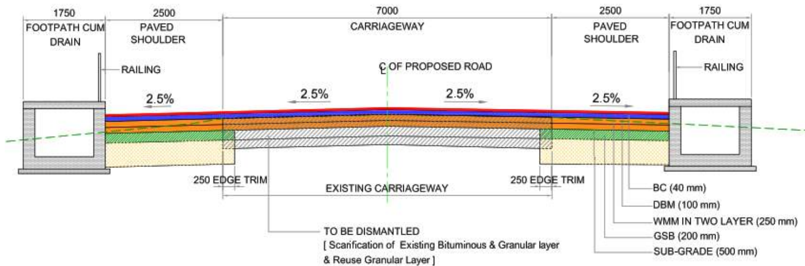
TCS- 1 :- TYPICAL CROSS SECTION OF TWO LANE CARRIAGEWAY WITH PAVED SHOULDER IN BUILT UP AREA WITH BOTH SIDE COVERED DRAIN CUM FOOTPATH IN PLAIN TERRAIN
