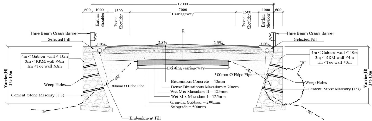
Type - 1A - Typical Cross-Section for Two Lane Carriageway With Paved Shoulder In Mountainous Terrain With Both Side Fill & Protection As Applicable (Reconstruction)
