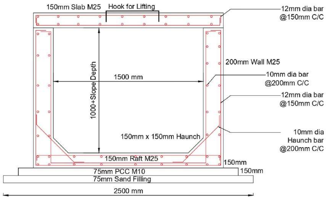
Section of Drain from TRTC Motor Stand to Gandacherra Junction
