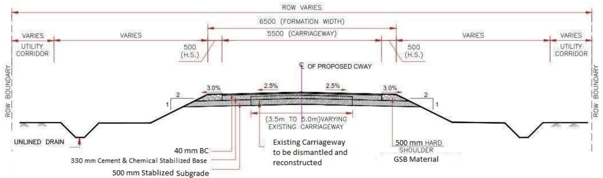
Type-I Reconstruction
