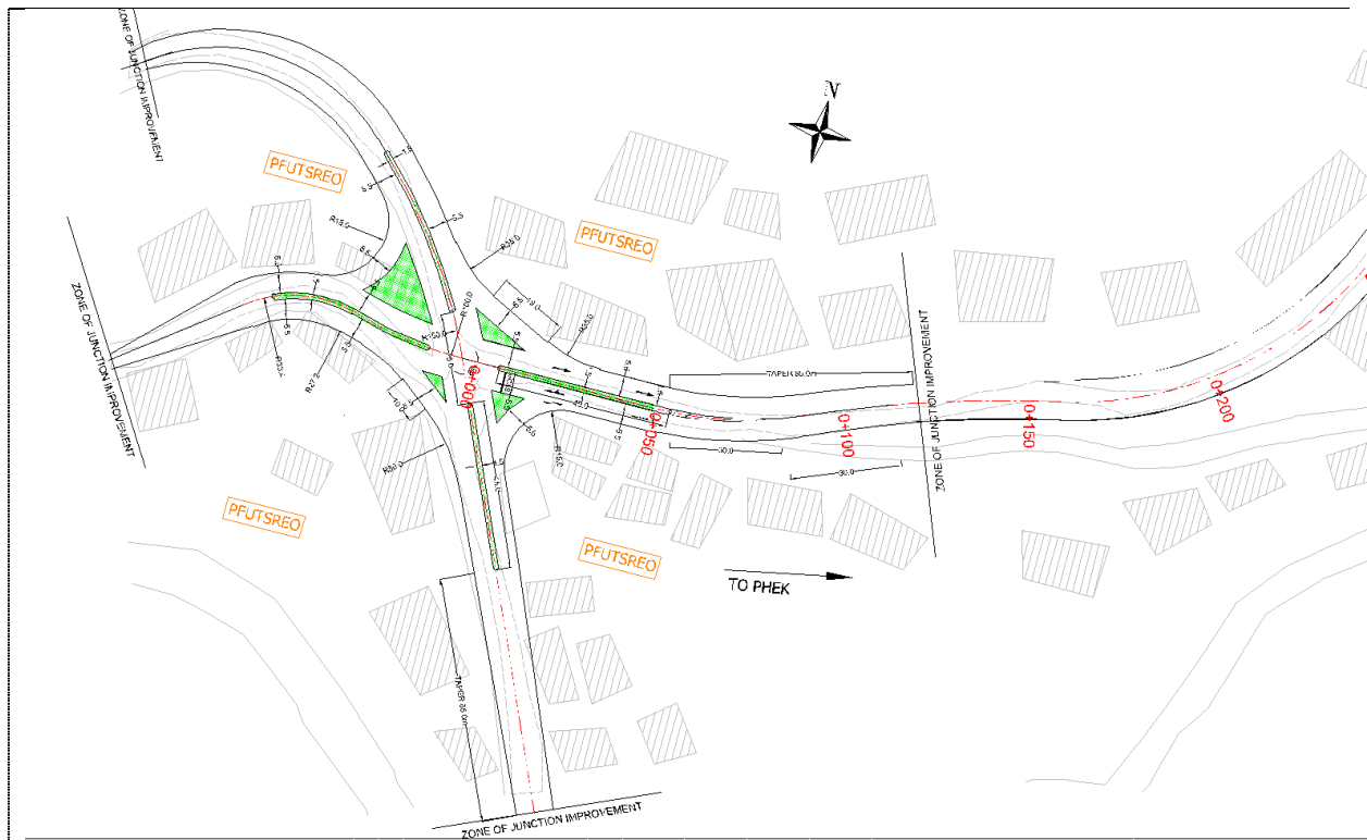
Figure B-7: Junction Improvement Proposal for Junction with NH 29 and P P Road at Km 0/000
