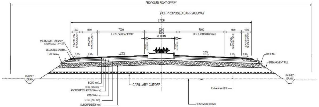
TCS-2: TYPICAL CROSS SECTION OF 4 LANE DIVIDED CARRIAGEWAY WITH PAVED SHOULDER IN BYPASS STRETCH
