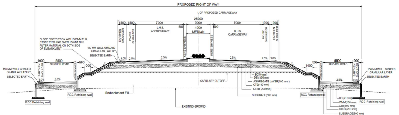
TCS-2A1: TYPICAL CROSS SECTION OF 4-LANE DIVIDED CARRIAGEWAY WITH BOTH SIDE SERVICE ROAD AND BOTH SIDE RETAINING WALL AND STONE PITCHING ALONG WITH BERM IN BYPASS STRETCH
