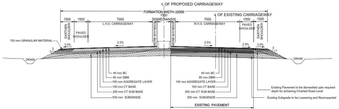
TCS-1D: TYPICAL CROSS SECTION OF 4 LANE DIVIDED CARRIAGEWAY WITH PAVED SHOULDER IN RURAL AREA (RECONSTRUCTION OVER EXISTING PAVEMENT )
