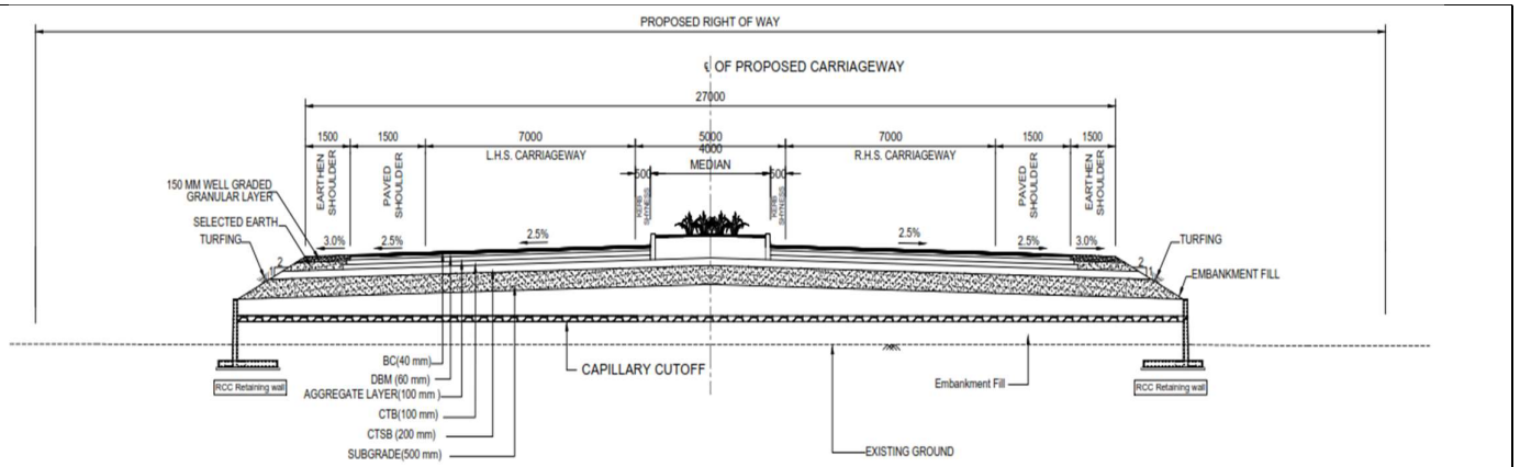
TCS-2C: TYPICAL CROSS SECTION OF 4 LANE DIVIDED CARRIAGEWAY WITH PAVED SHOULDER IN BYPASS STRETCH WITH BOTH SIDE RETAINING WALL
