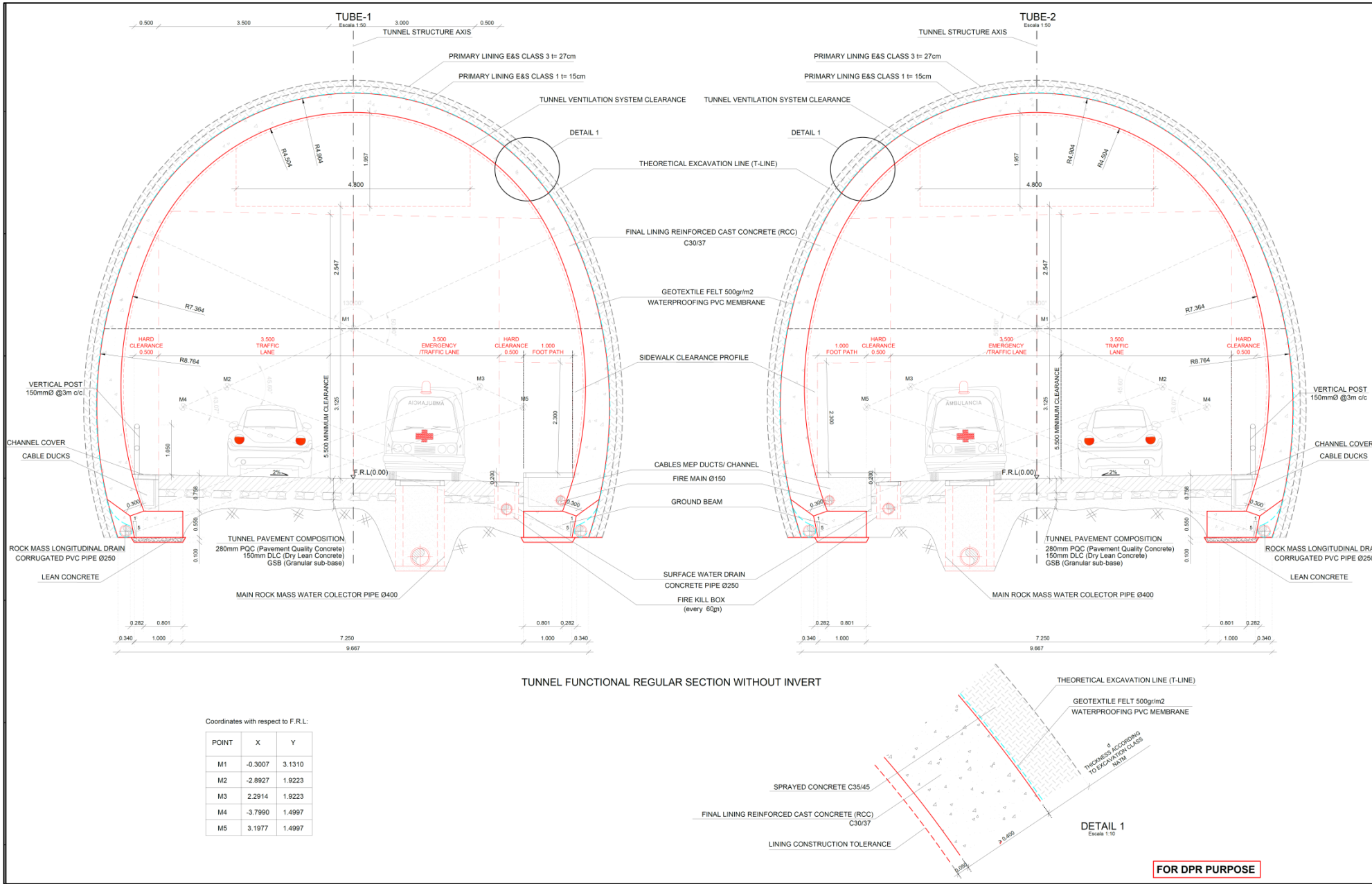
Tunnel-2 Uni-directional Tunnel Cross Section without invert
