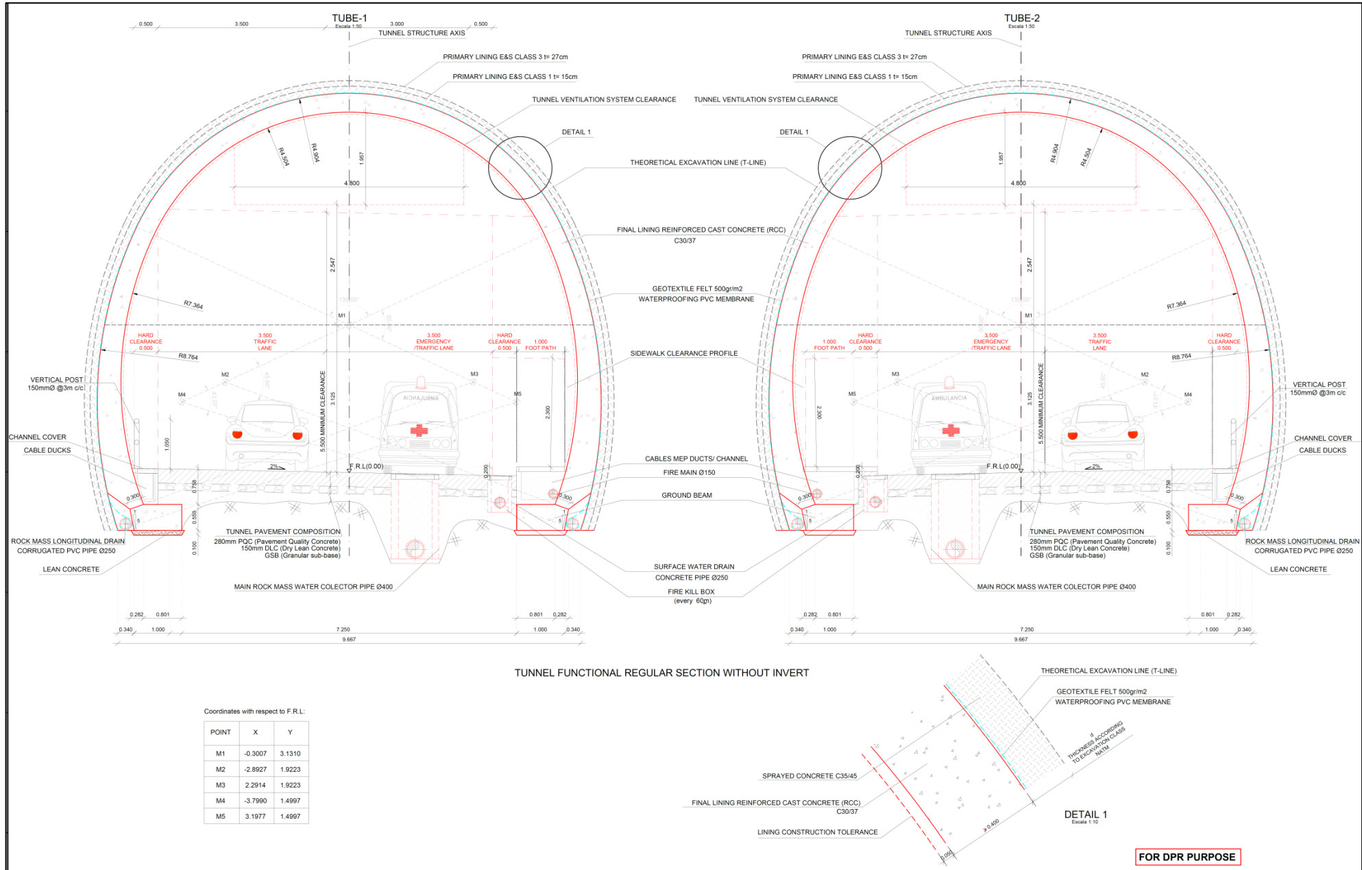
Tunnel-1 Uni-directional Tunnel Cross Section without invert
