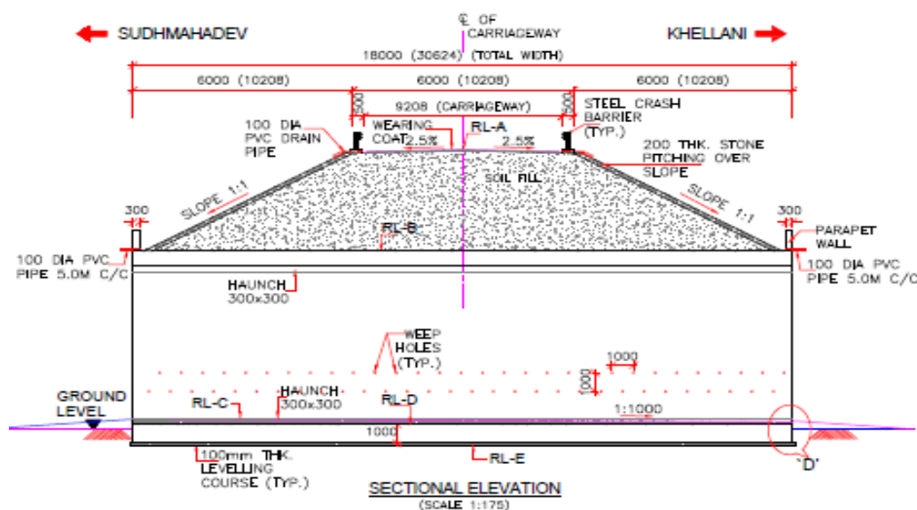
Overpass section
