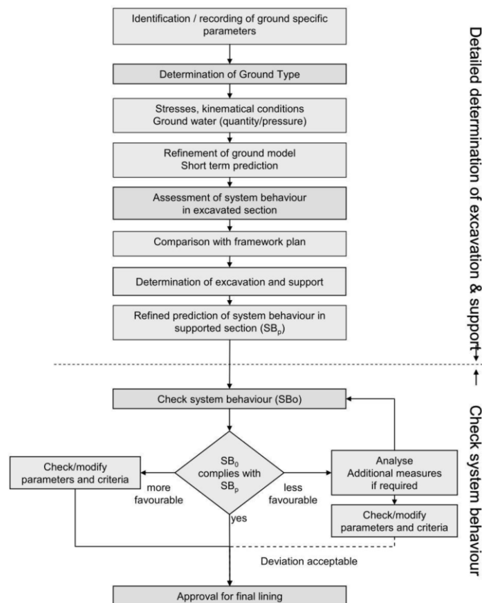
Figure 1: Basic procedure of determination of construction measures and check of system behaviour during construction (SBp = predicted system behaviour, SBo = observed system behaviour) from Austrian “Guideline for the Geotechnical Design of Underground Structures with Conventional Excavation” by the Austrian Society for Geomechanics
