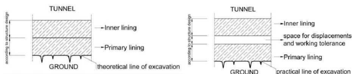
Figure 2 Schematic sketch of the geometrical condition for the definition of the line of excavation
