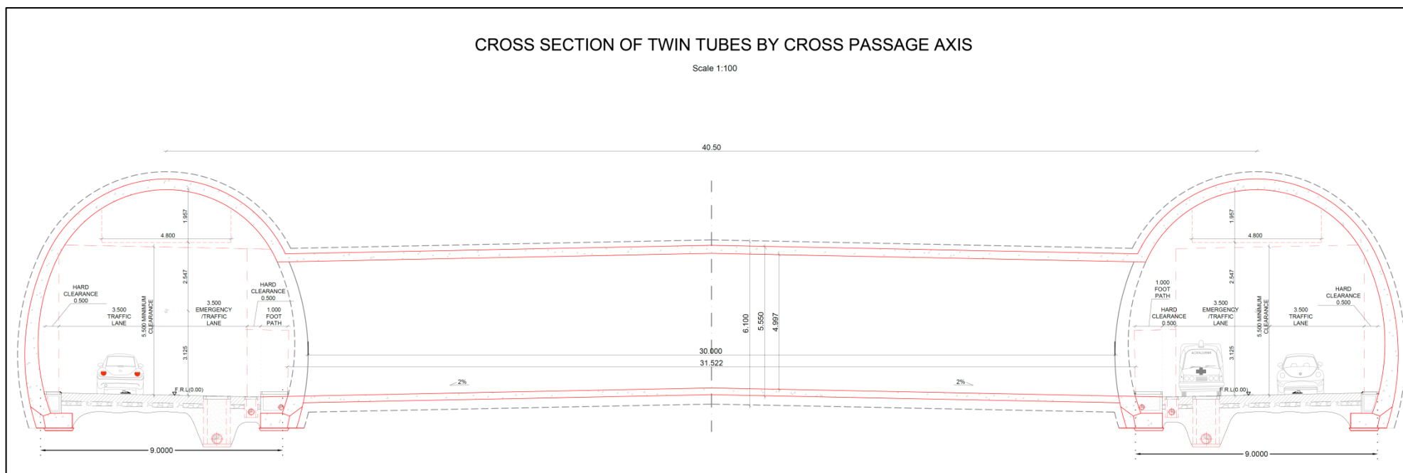
Cross-Section For Cross- Passage
