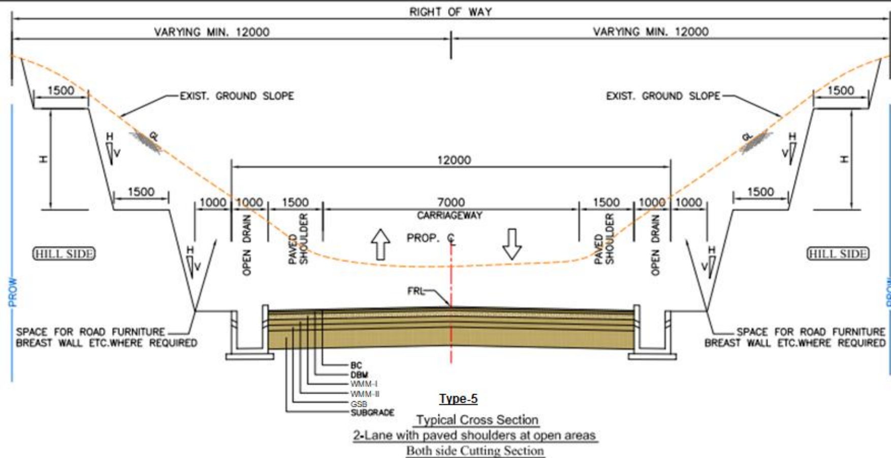
Fig 2.13: Typical Cross-Section
