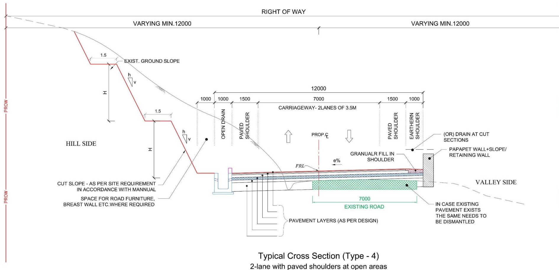
Fig 2.12: Typical Cross-Section
