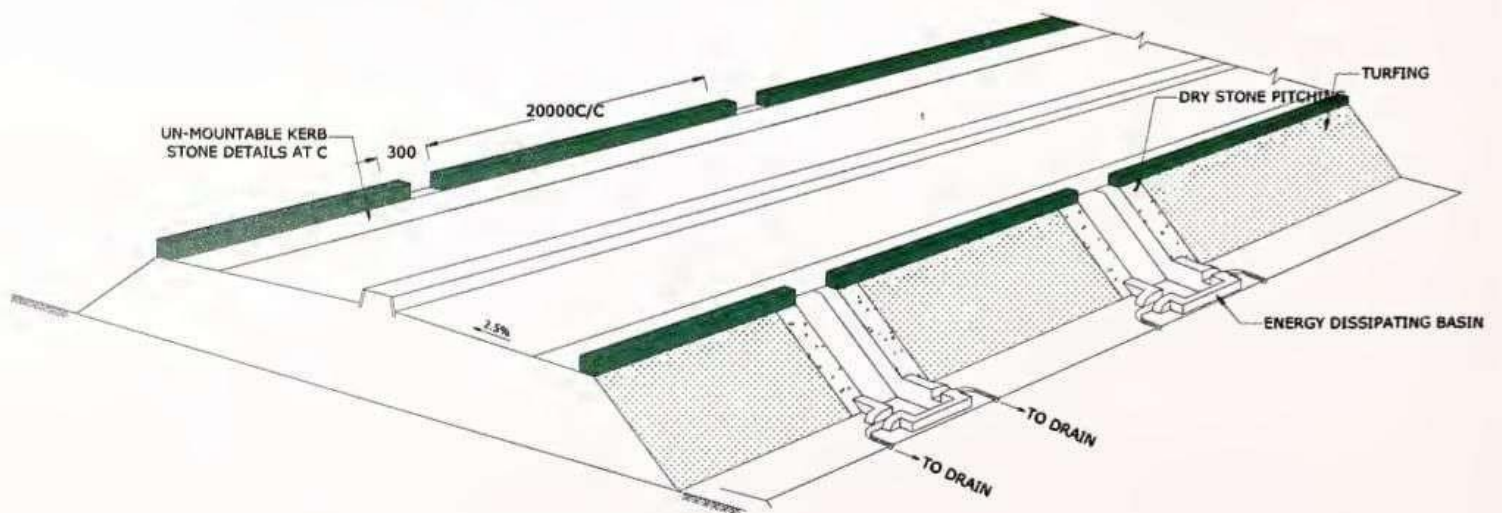
Fig. 4.23 A Schematic View of Slope Protection Arrangement with Plain Chute/Flume
