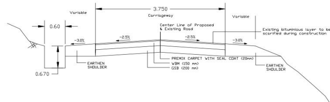
Existing Pavement
