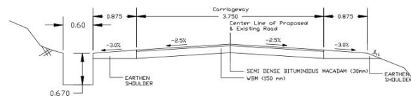
Proposed Pavement
