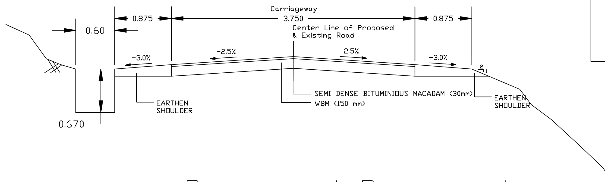
Proposed Pavement
