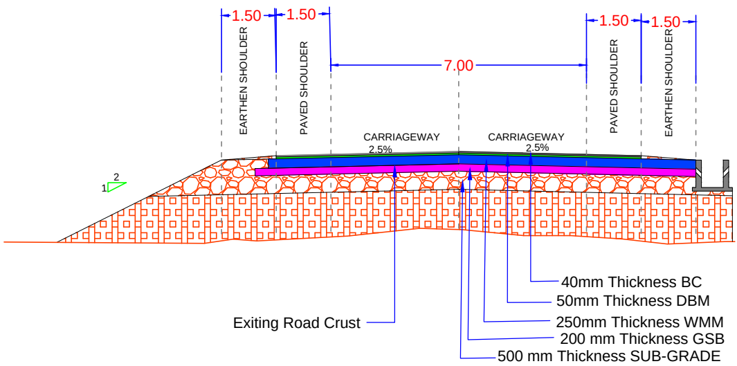
TCS -13 A (Improvement Section)
