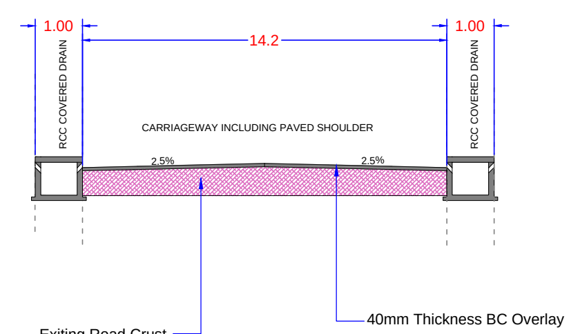
TCS -08 (BC Overlay Section)
