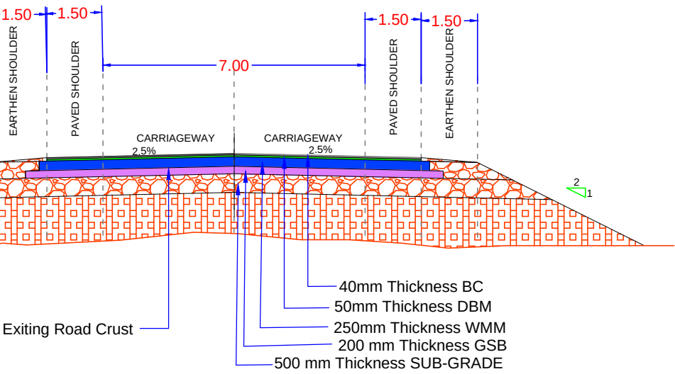
TCS -5 B (Improvement Section)
