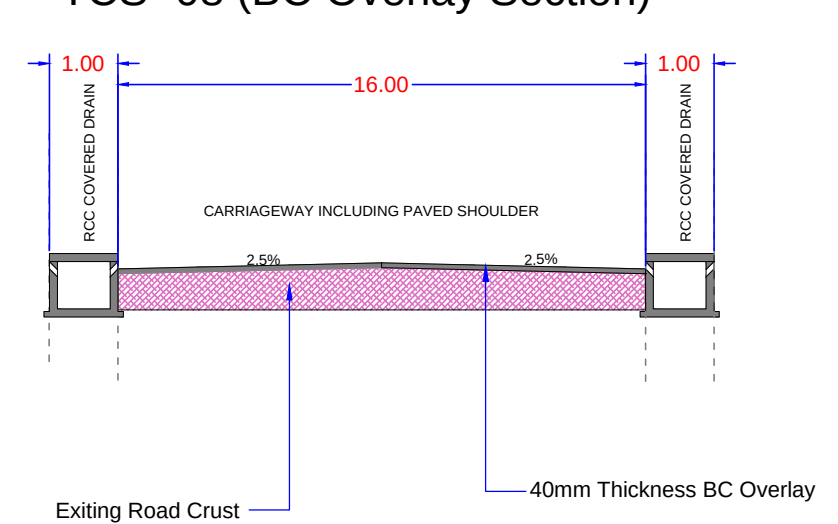
TCS -11 (BC Overlay Section)
