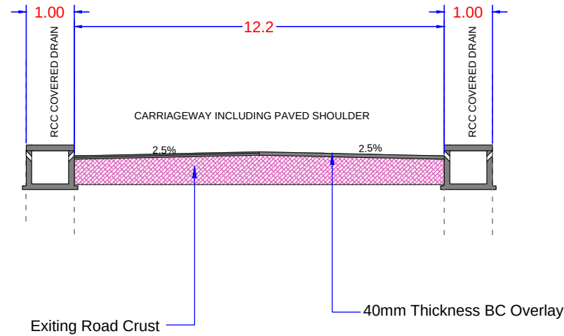
TCS -09 (BC Overlay Section)
