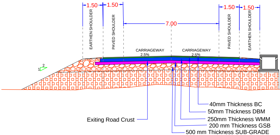
TCS -15 A (Improvement Section)
