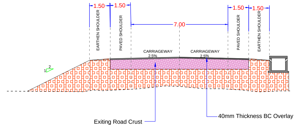
TCS -15 (BC Overlay Section)
