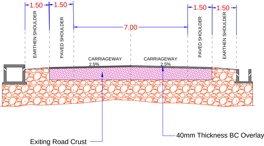
TCS -16 (BC Overlay Section)
