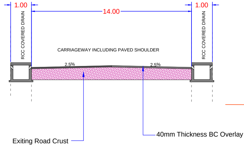
TCS -12 (BC Overlay Section)
