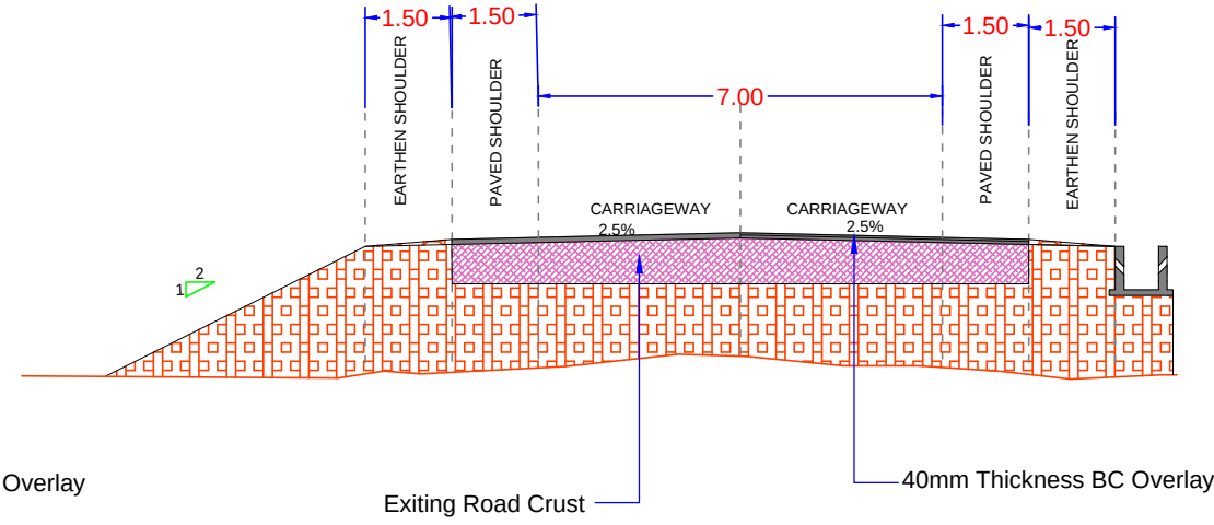
TCS -13 (BC Overlay Section)
