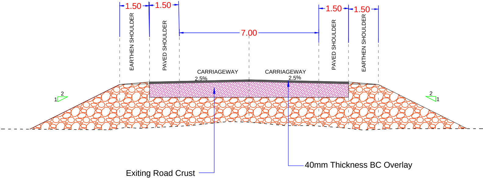
TCS -05 (BC Overlay Section)
