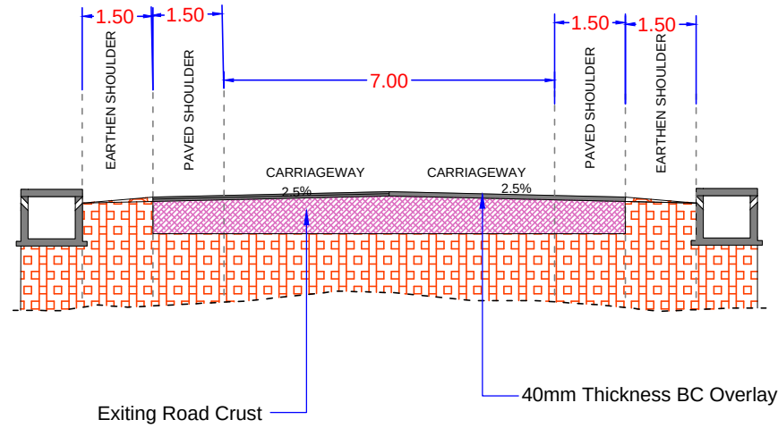
TCS -10 (BC Overlay Section)
