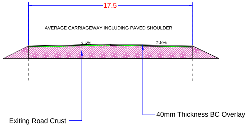
TCS -04 BC Overlay Section
