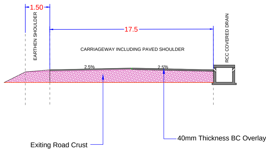
TCS -06 (BC Overlay Section)
