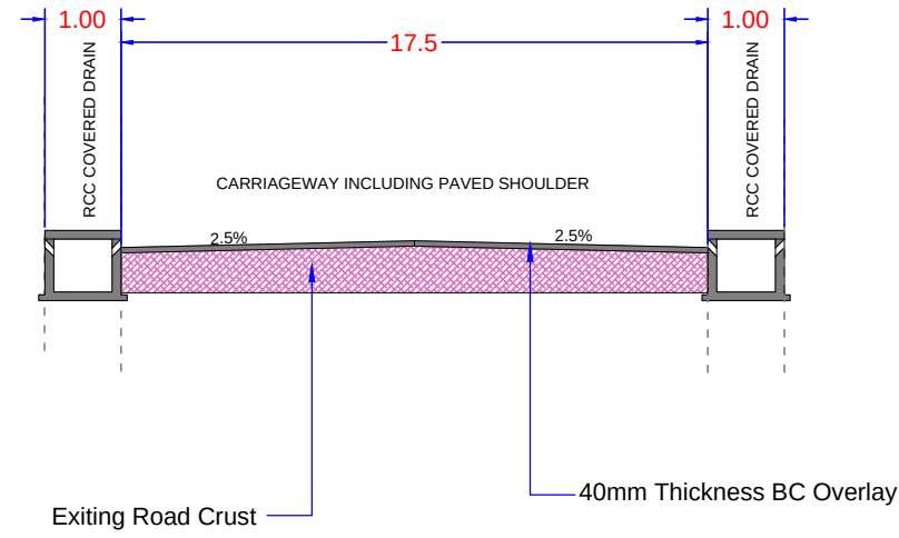
TCS -07 (BC Overlay Section)
