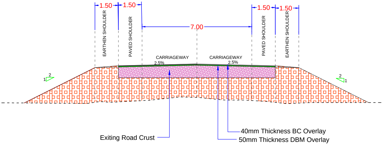
TCS -5 A BC & DBM Overlay Section
