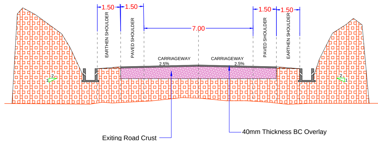
TCS -14 (BC Overlay Section)
