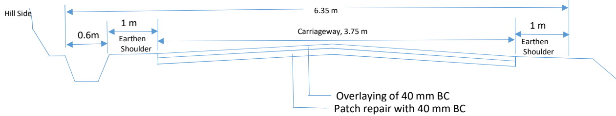
TYPICAL CROSS SECTION-1 (TCS-3) SHOWING ROAD FEATURES PAVEMENT DETAILS
