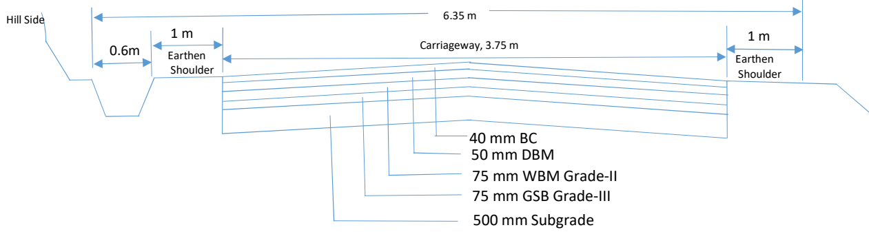
TYPICAL CROSS SECTION-1 (TCS-1) SHOWING ROAD FEATURES PAVEMENT DETAILS
