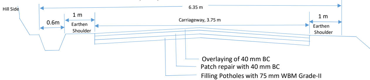
TYPICAL CROSS SECTION-1 (TCS-2) SHOWING ROAD FEATURES PAVEMENT DETAILS
