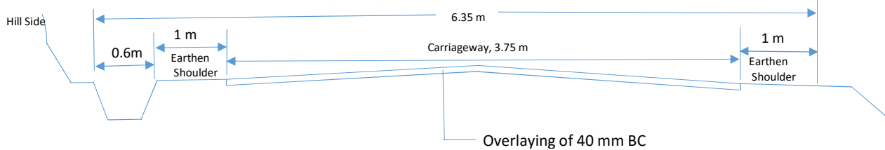
TYPICAL CROSS SECTION-1 (TCS-4) SHOWING ROAD FEATURES PAVEMENT DETAILS
