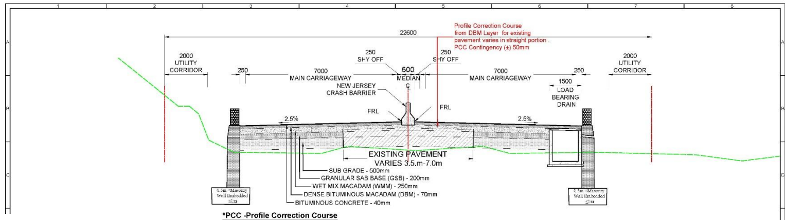
TYPICAL CROSS SECTION-09 CONCENTRIC WIDENING OF FOUR LANE IN HILL AREA WITH LOAD BEARING DRAIN BUILT-UP AREA
