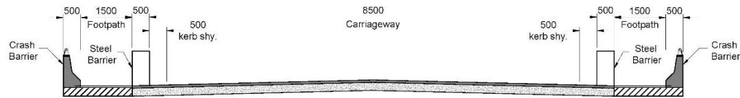
TYPICAL CROSS SECTION-12 NEW CONSTRUCTION OF BRIDGE AT VAILOO ROAD JUNCTION
