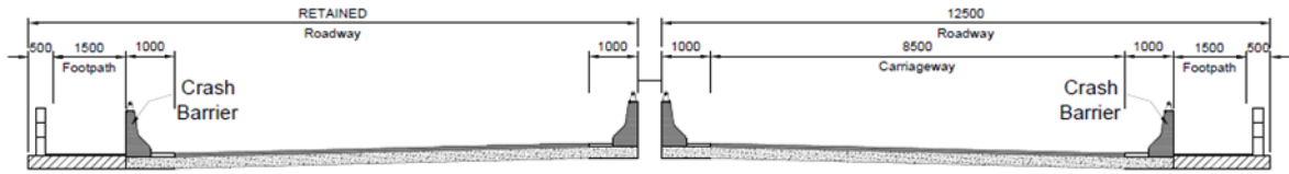
TYPICAL CROSS SECTION-11 ECCENTRIC BRIDGE WIDENING OF FOUR LANE IN HILL AREA
