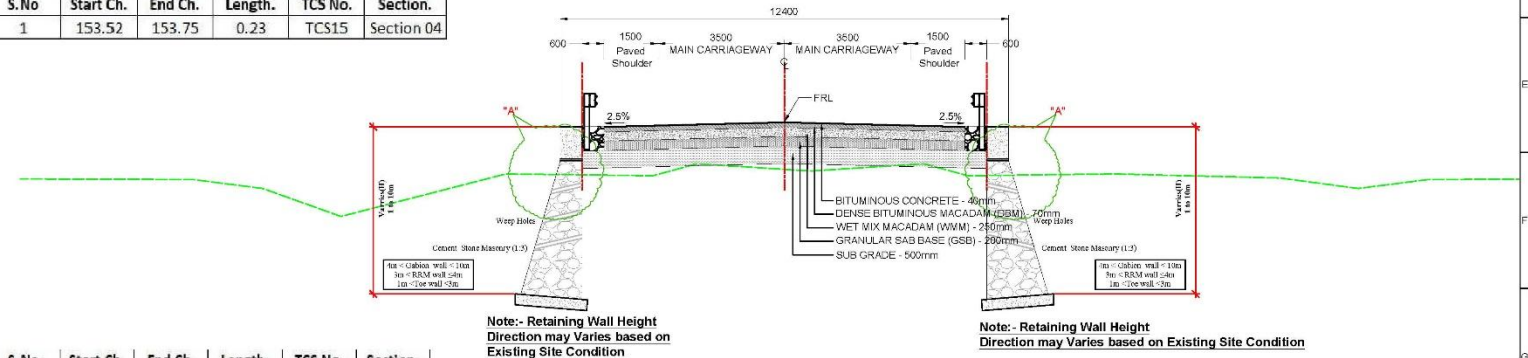
TYPICAL CROSS SECTION-16 TWO LANE BRIDGE APPROACH SECTION DOWN STREAM SIDE Note:- Retaining Wall Height Direction may Varies based on Existing Site Condition
