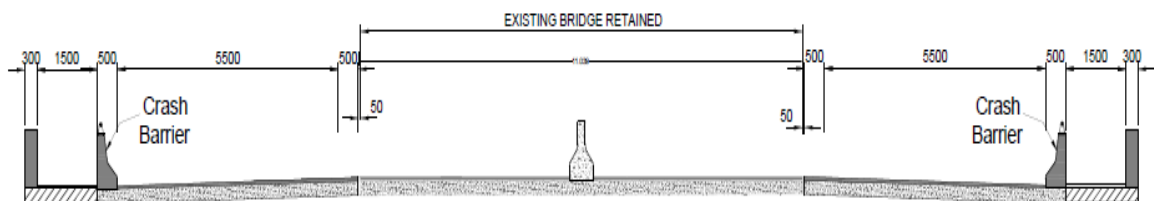
TYPICAL CROSS SECTION-010 CONCENTRIC WIDENING ON BOTH HAND SIDE SINGLE LANE BRIDGE BUILT-UP AREA
