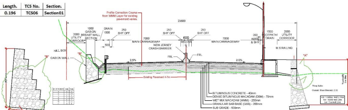
TYPICAL CROSS SECTION-06 ECCENTRIC WIDENING OF FOUR LANE IN HILL AREA LHS SIDE ALONG WITH PROTECTION WORKS BOTH SIDE
