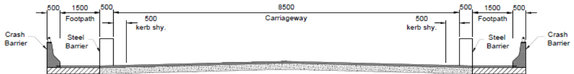
TYPICAL CROSS SECTION-12 NEW CONSTRUCTION OF BRIDGE AT VAILOO ROAD JUNCTION
