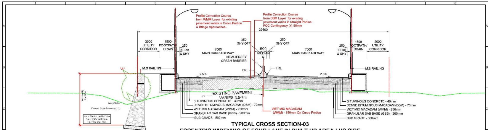
TYPICAL CROSS SECTION-03 ECCENTRIC WIDENING OF FOUR LANE IN BUILT-UP AREA LHS SIDE
