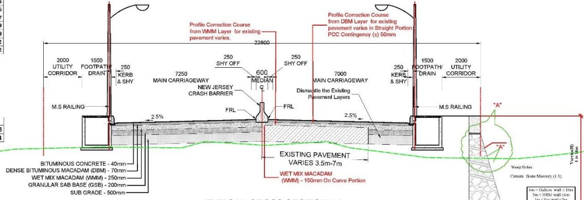
TYPICAL CROSS SECTION-04 ECCENTRIC WIDENING OF FOUR LANE IN BUILT-UP AREA RHS SIDE
