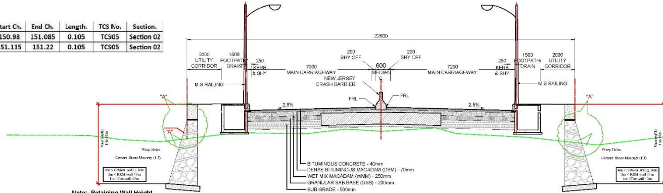
TYPICAL CROSS SECTION-05 CONCENTRIC WIDENING OF FOUR LANE IN BUILT-UP AREA PROTECTION WORK BOTH SIDE
