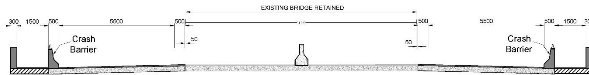
TYPICAL CROSS SECTION-010 CONCENTRIC WIDENING ON BOTH HAND SIDE SINGLE LANE BRIDGE BUILT-UP AREA
