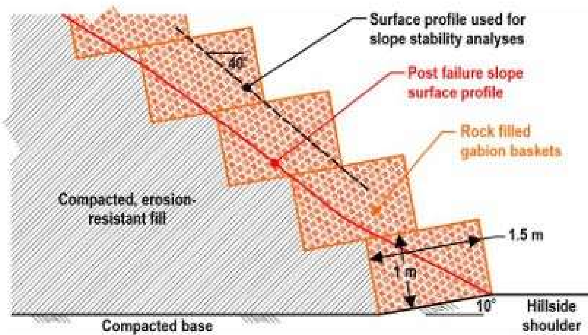
Figure 4. Placement of rock filled gabion baskets
