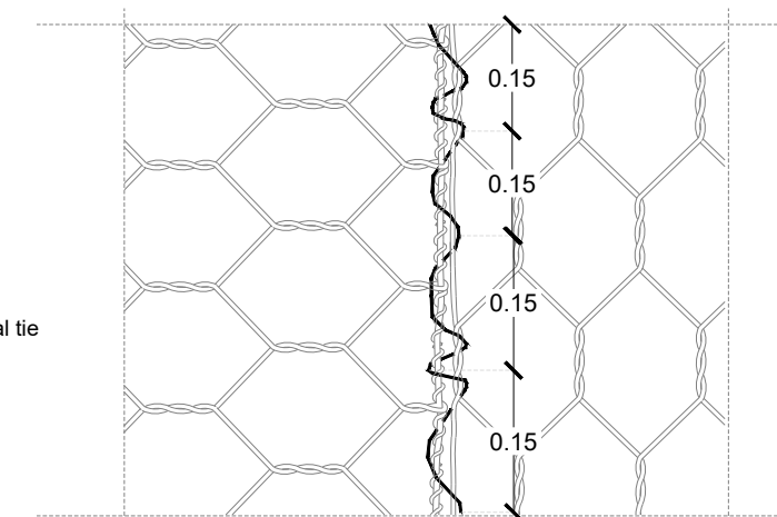
LACING DETAIL
