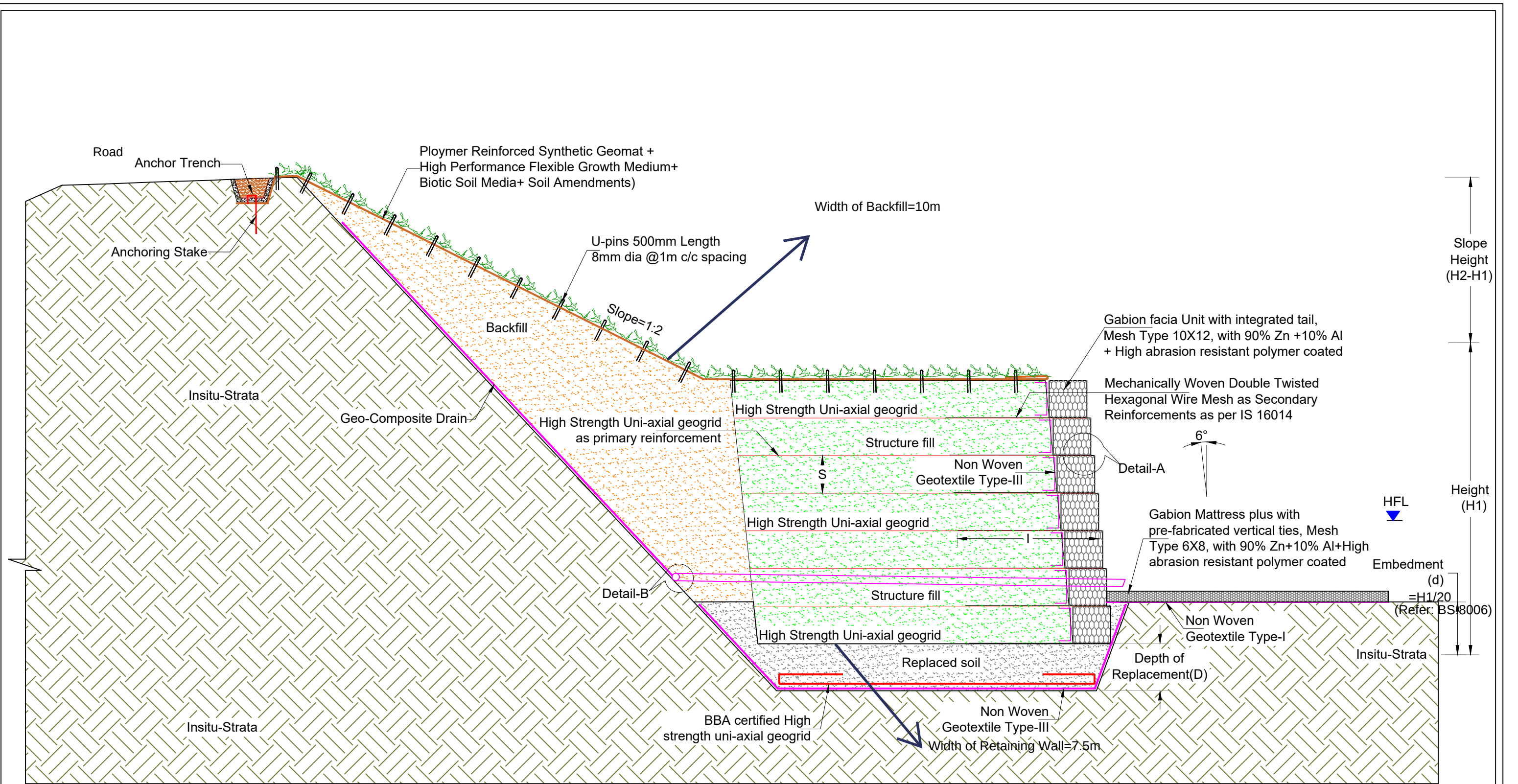
TCS-2A TYPICAL CROSS SECTION OF SLOPE PROTECTION MEASURES USING PARAMESH SYSTEM AND SYNTHETIC GEOMAT
