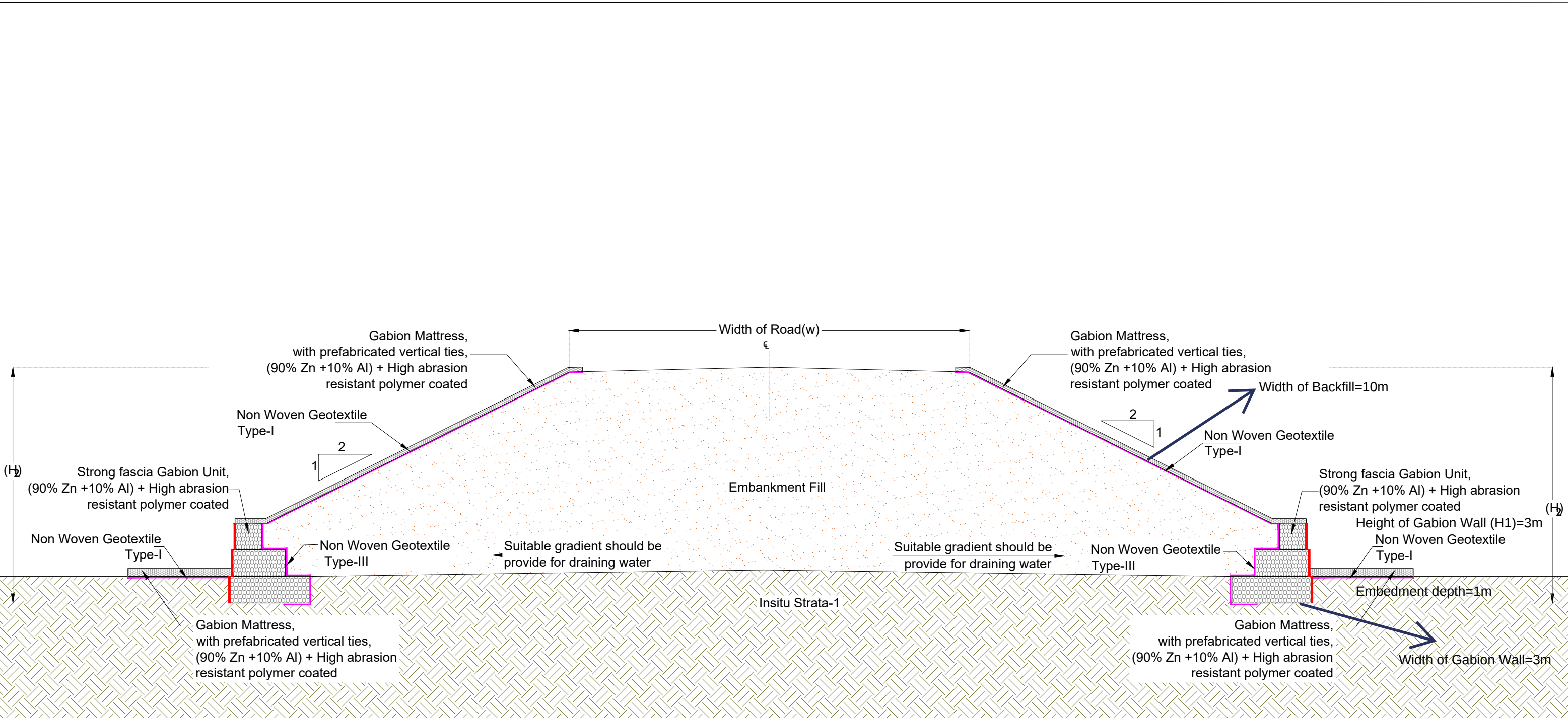
TCS-3 TYPICAL CROSS SECTION OF EMBANKMENT PROTECTION AT POND LOCATION
