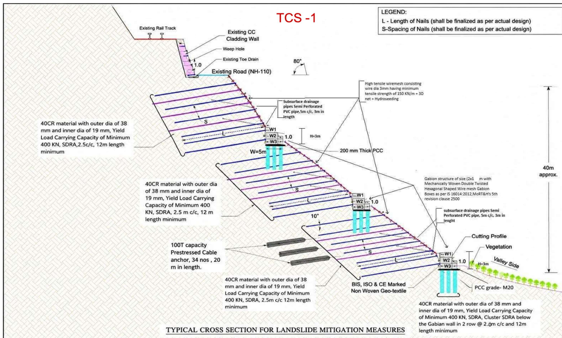
Drawing - TCS - 01
