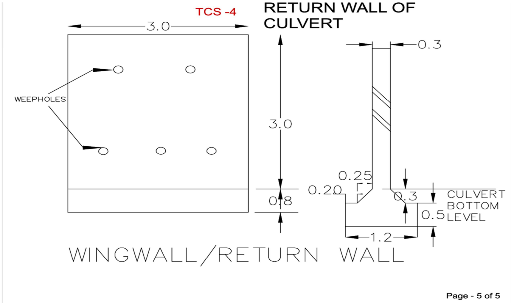
Return wall of Culvert - TCS - 4
