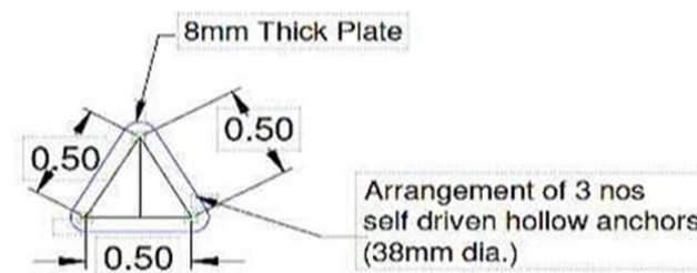
TYPICAL ARRANGEMENT OF SDR CLUSTER (DETAILS-1)
