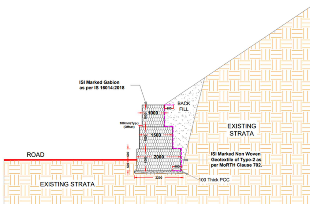
TYPICAL CROSS SECTION OF TOE BREAST WALL USING GABION
