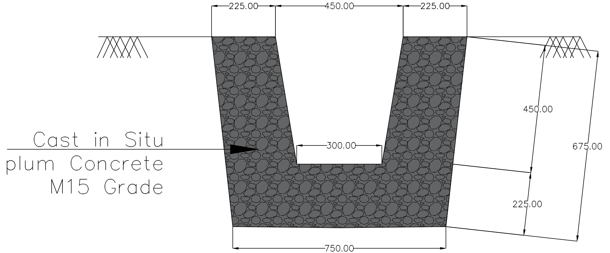
X-Section for Construction of lined Drain
