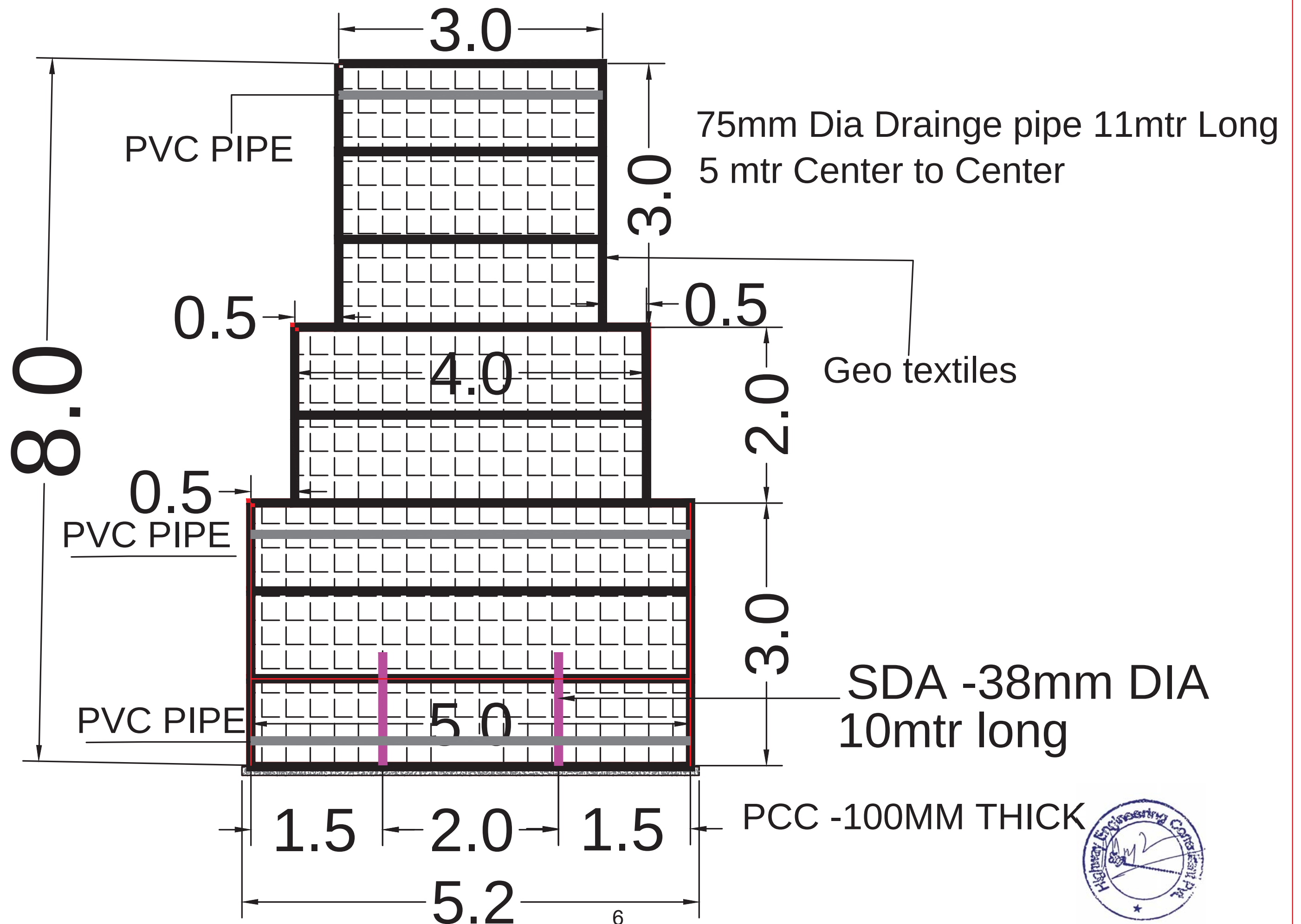
GABION WALL SECTION AT NANDAPRYAG
